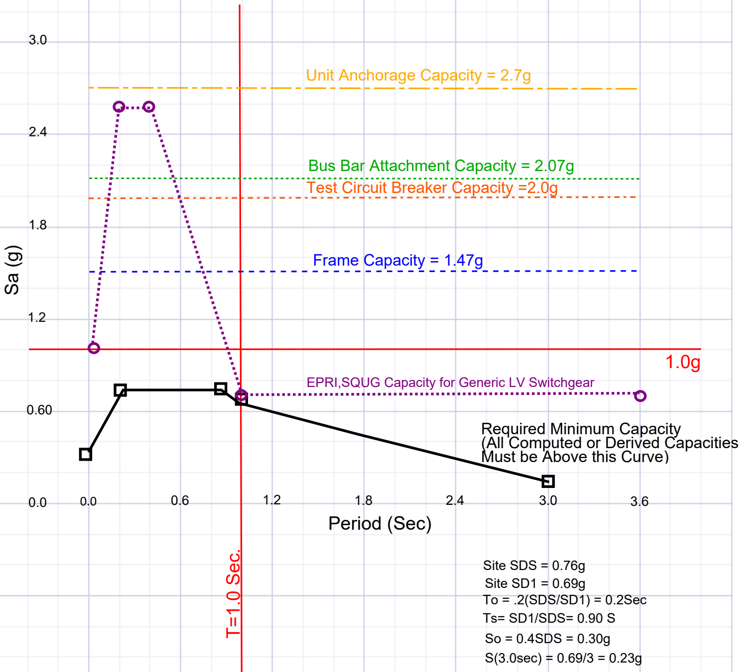
FIGURE 1.1 BOUNDING SPECTRAL CAPACITIES OF TRYSTAR DOCKING GEAR AT THE SLCAP TRP: SEISMIC CERTIFICATION COMPLIANCE HAS BEEN VERIFIED BY INDICATED COMPONENT CAPACITIES BEING GREATER THAN REQUIRED MINIMUM RESPONSE SPECTRUM
